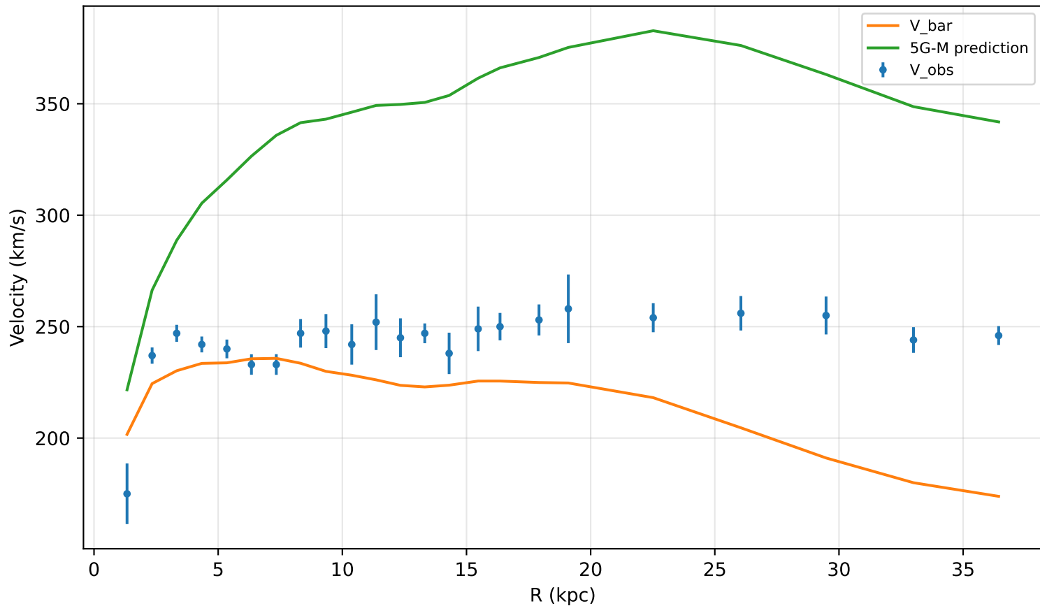
Worst-case check: NGC6195
