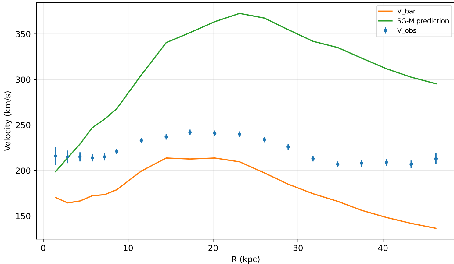
Worst-case check: NGC5371
