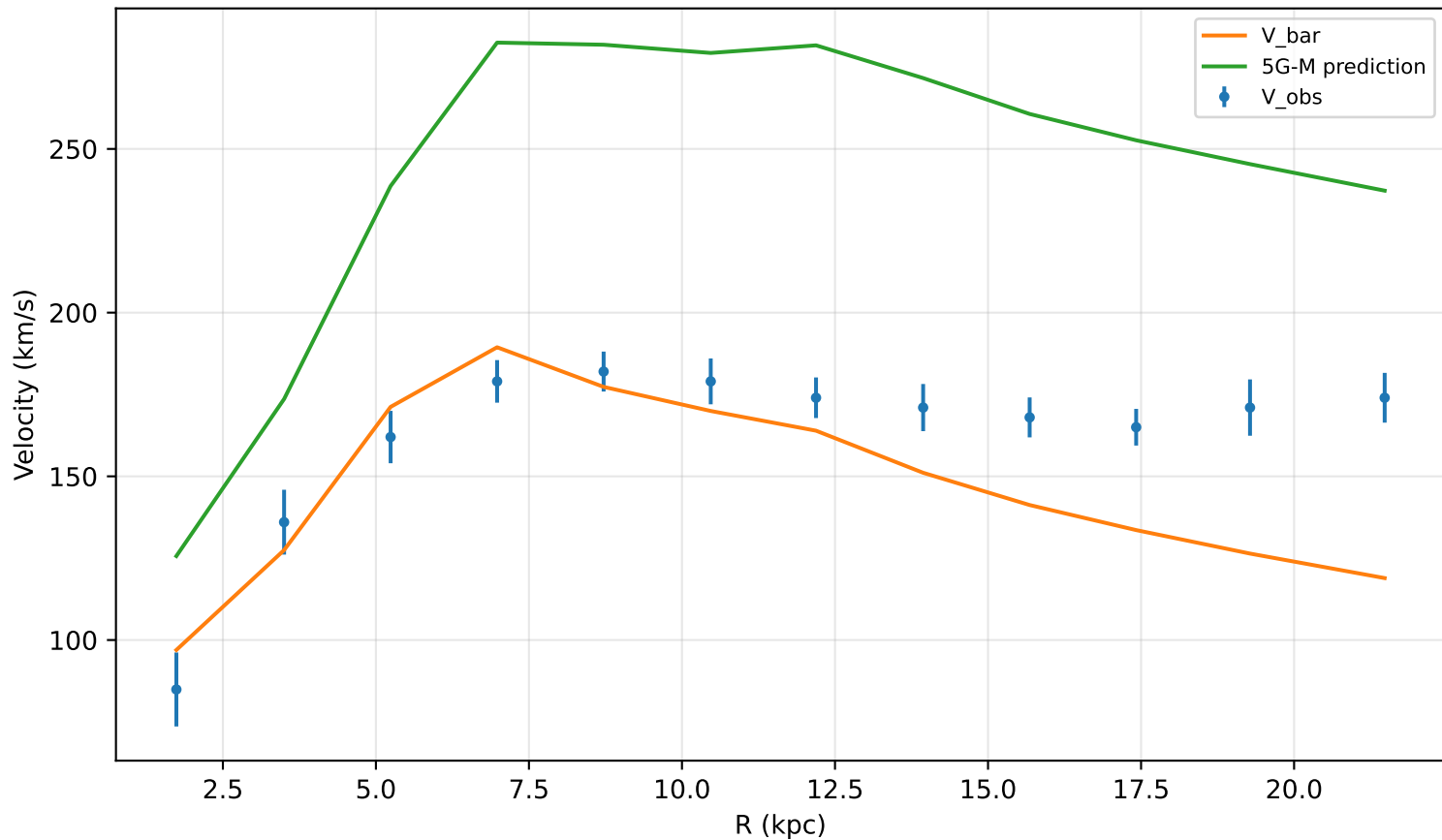
Worst-case check: NGC4088
