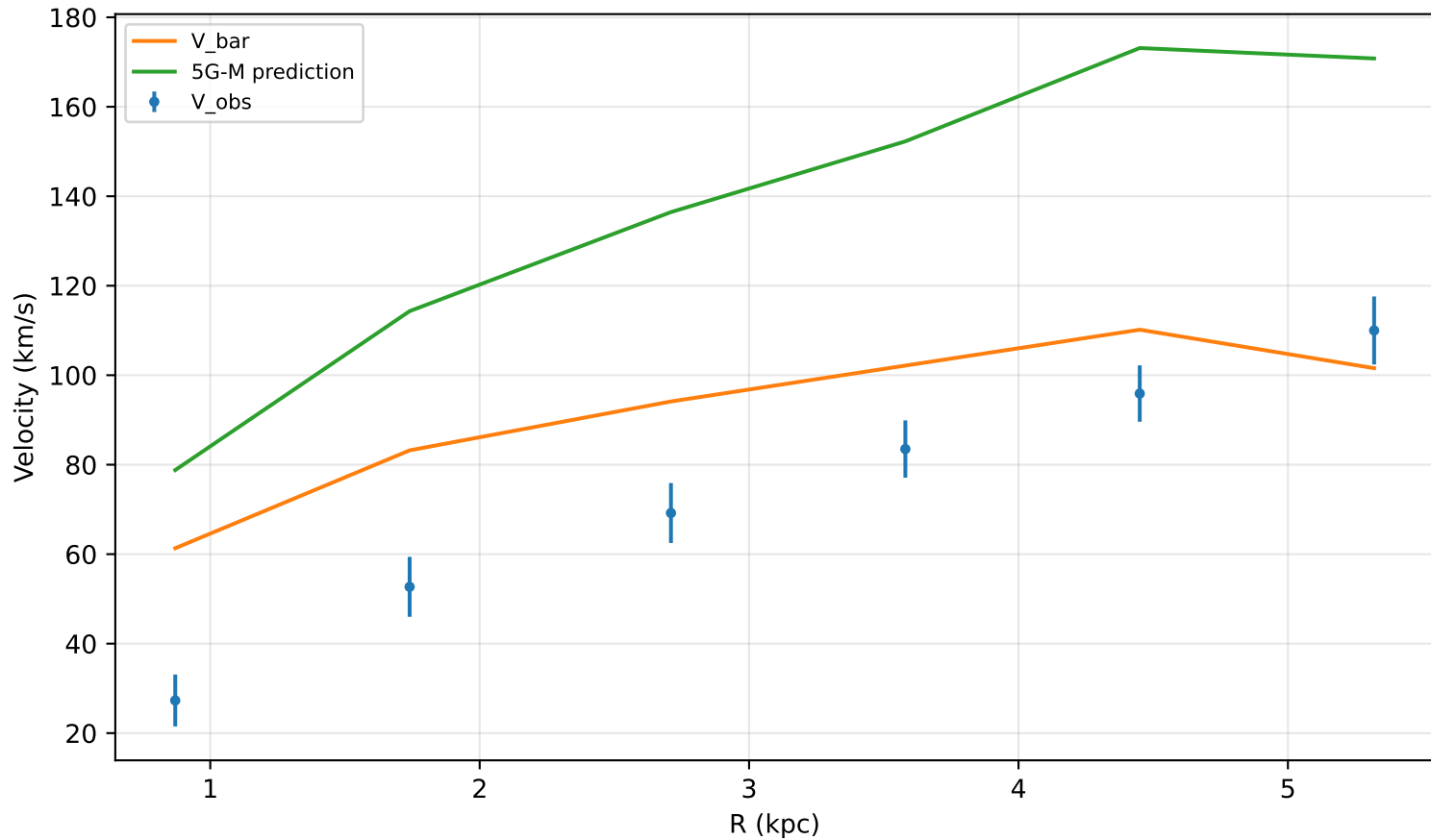
Worst-case check: NGC4389
