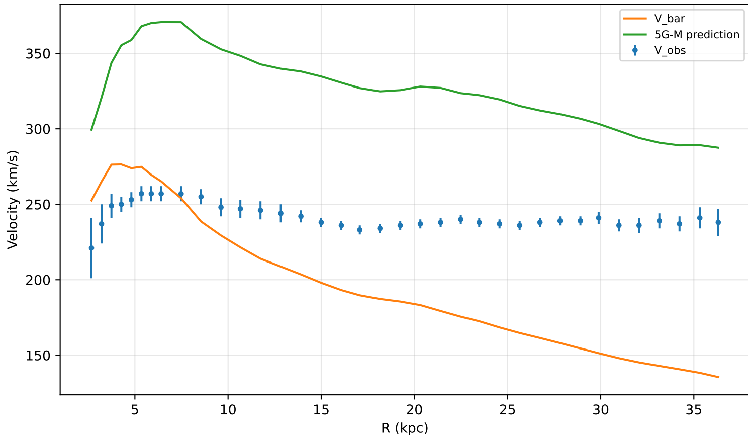
Worst-case check: NGC7331
