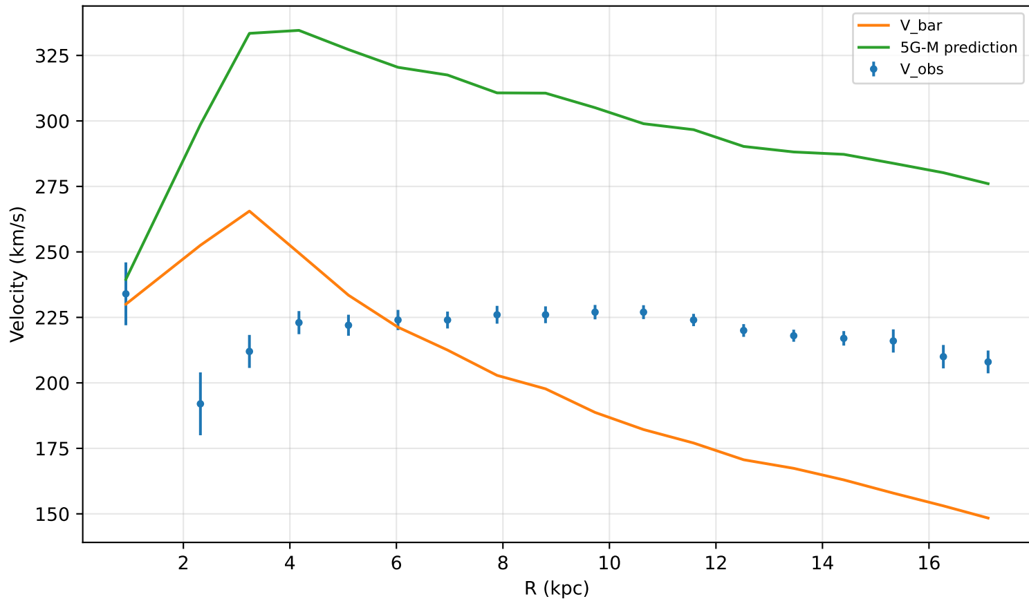
Worst-case check: NGC0891
