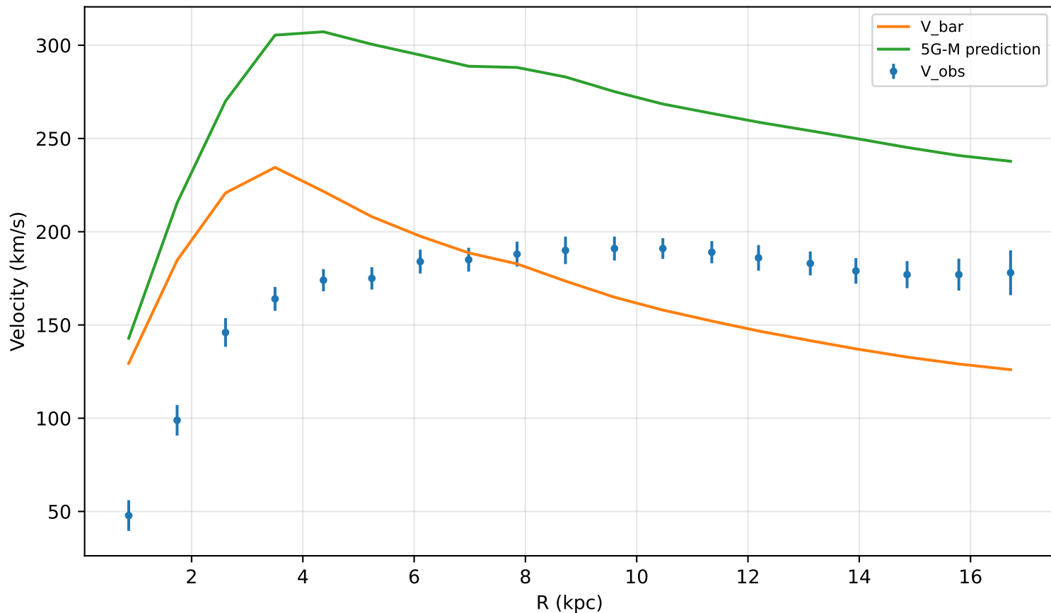
Worst-case check: NGC4217
