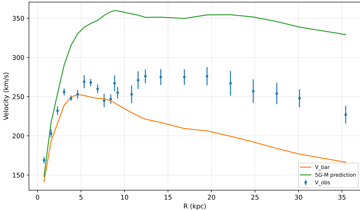
Worst-case check: NGC2955
