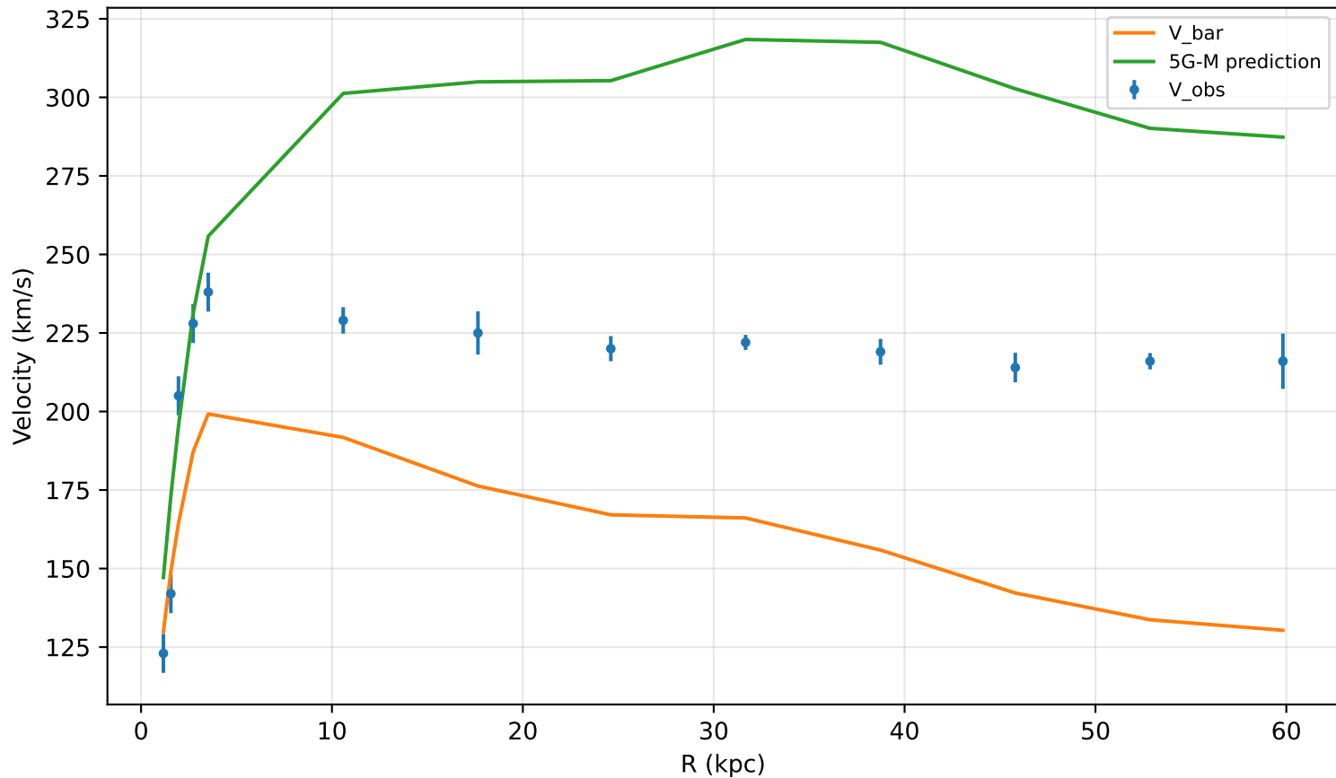
Worst-case check: NGC0801
