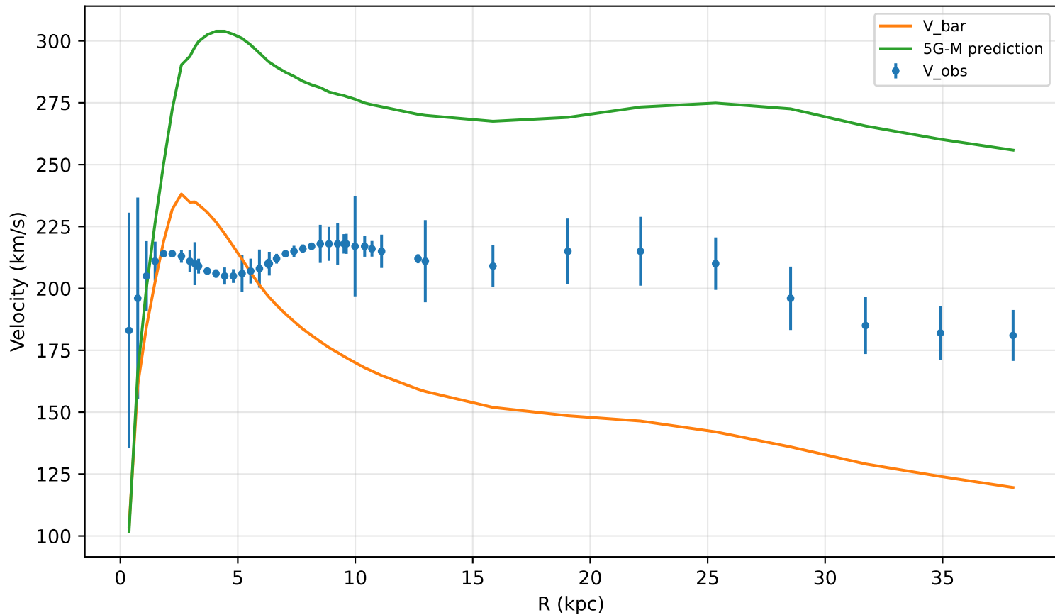
Worst-case check: UGC02916
