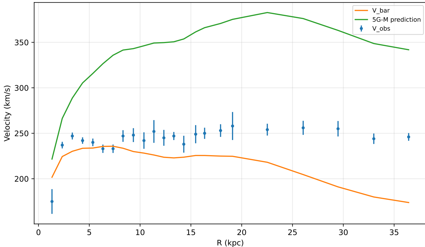
Worst-case check: NGC6195
