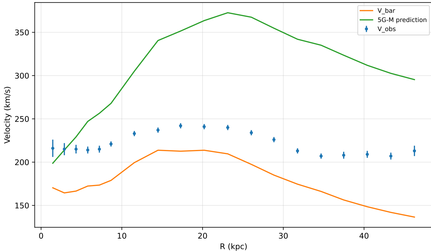
Worst-case check: NGC5371
