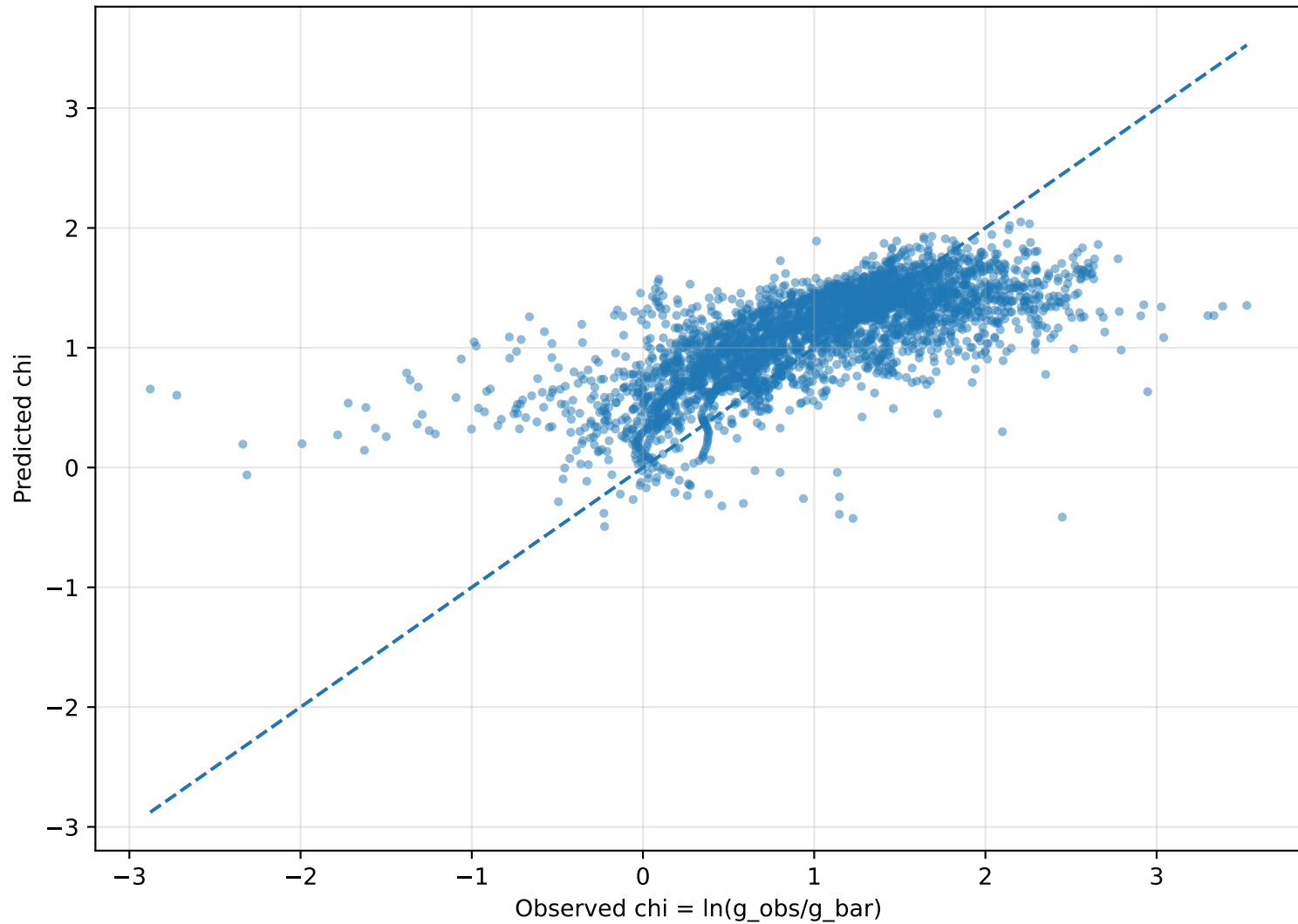
5G-M full-sample metric reconstruction check
