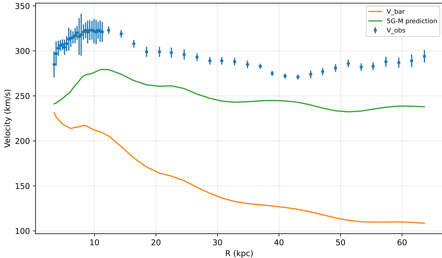
Worst-case check: NGC2841
