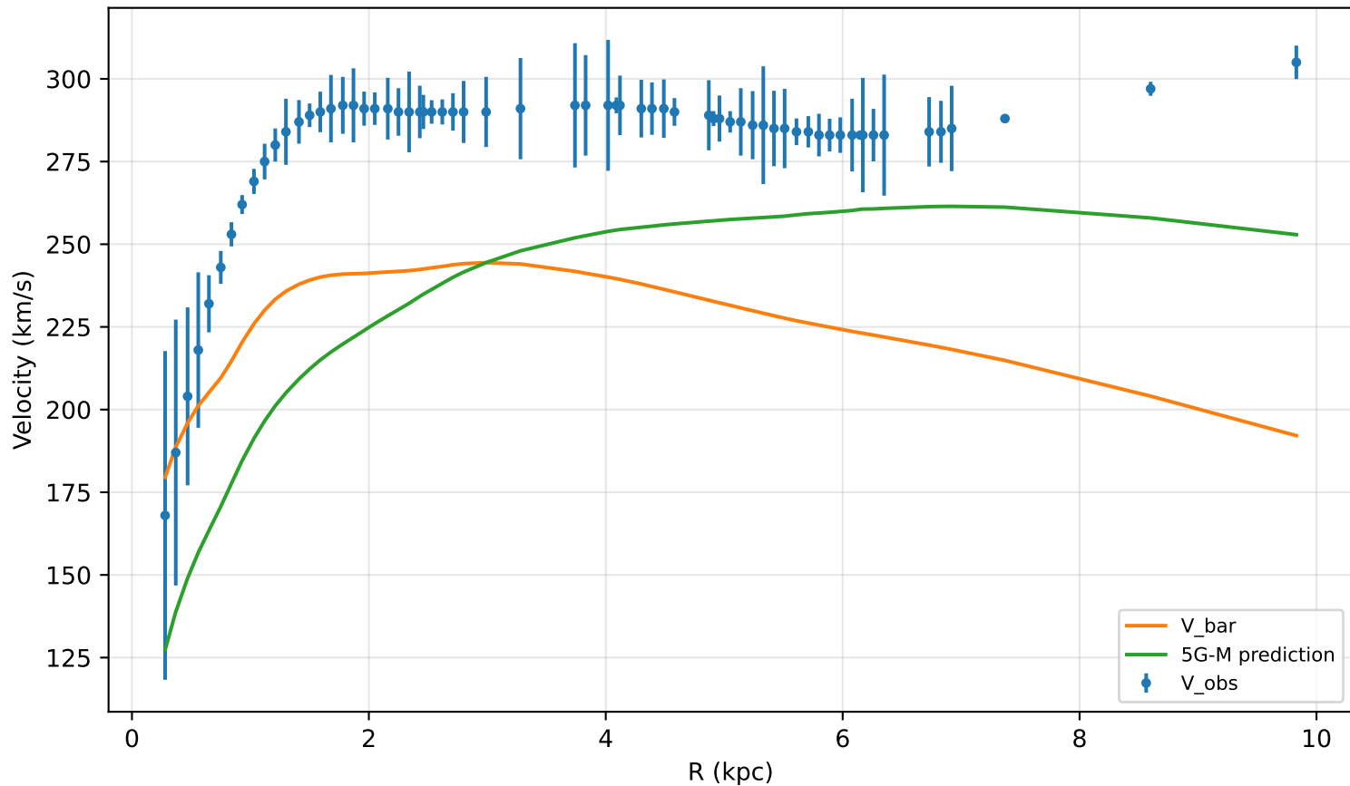
Worst-case check: UGC11914
