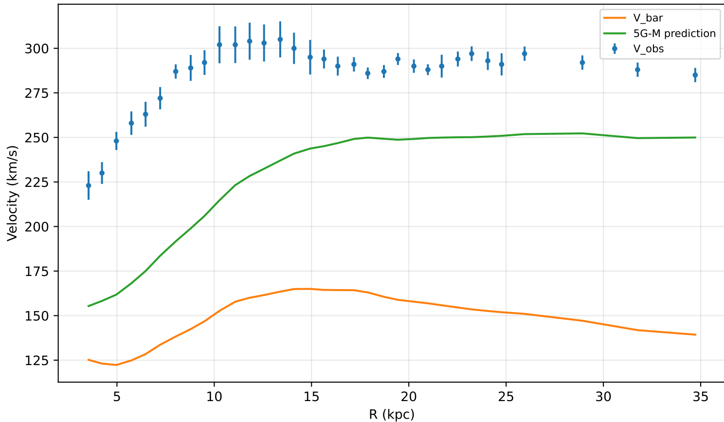
Worst-case check: NGC5985
