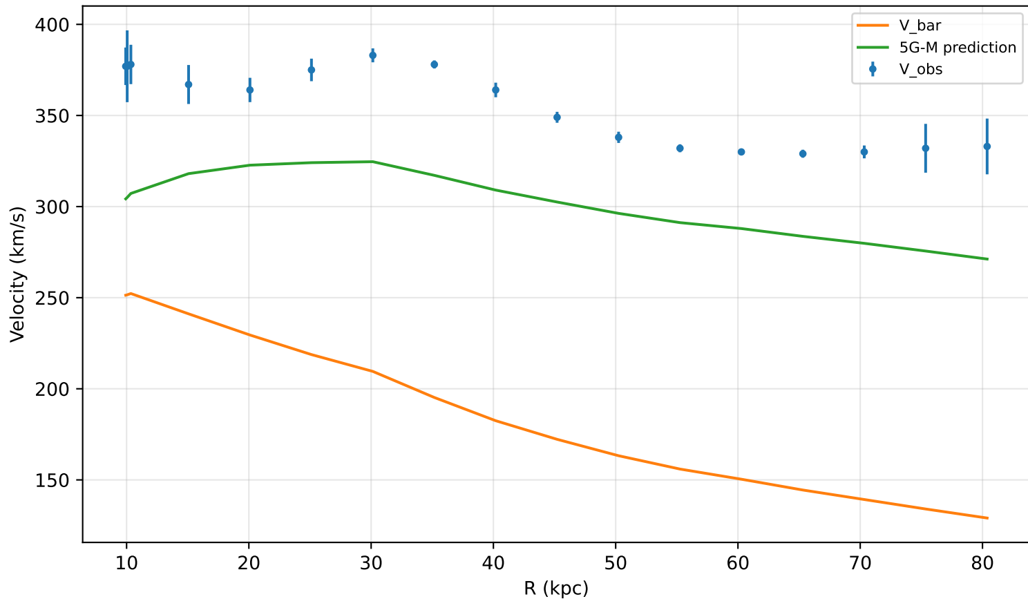
Worst-case check: UGC02487
