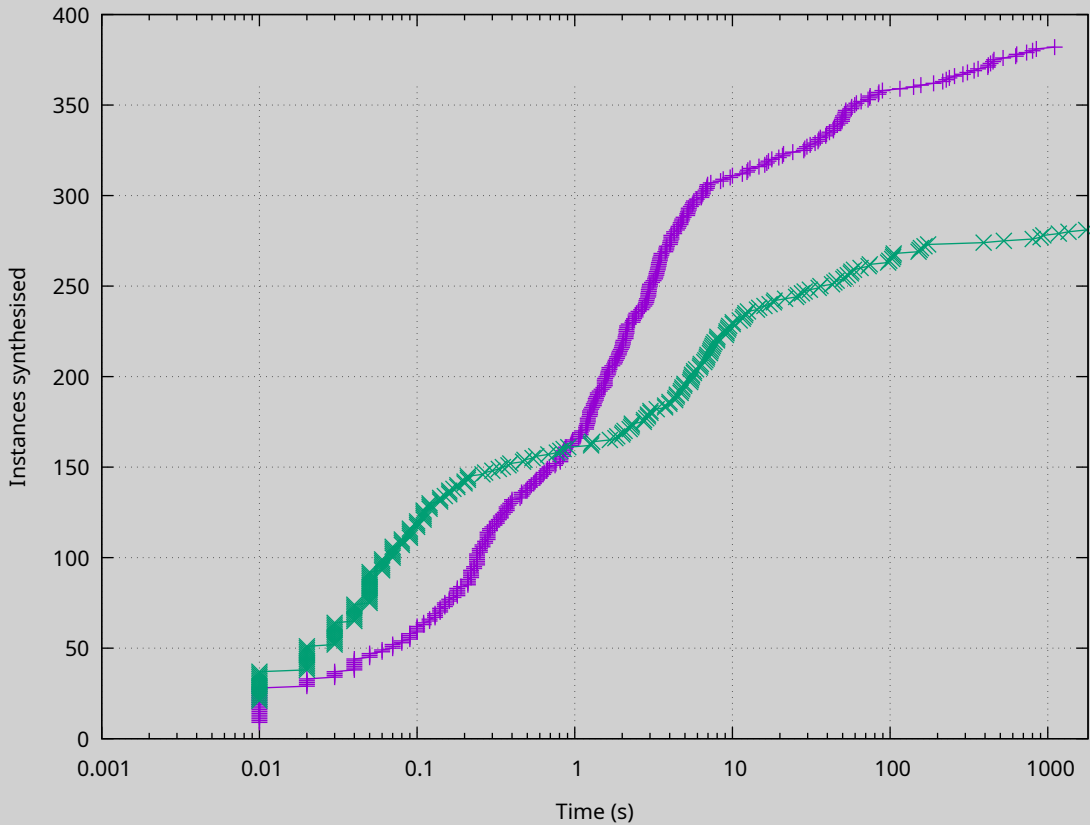
Arjun synthesis CDF: instances solved vs. time
