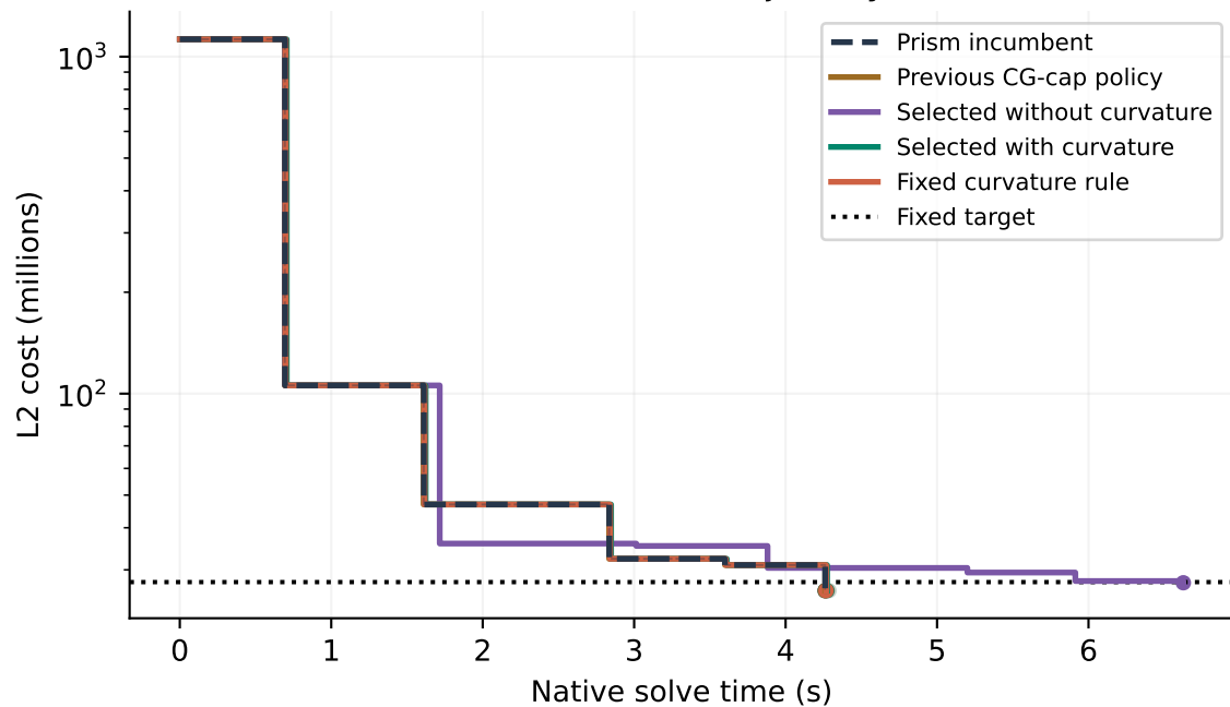
Recorded full trajectory
