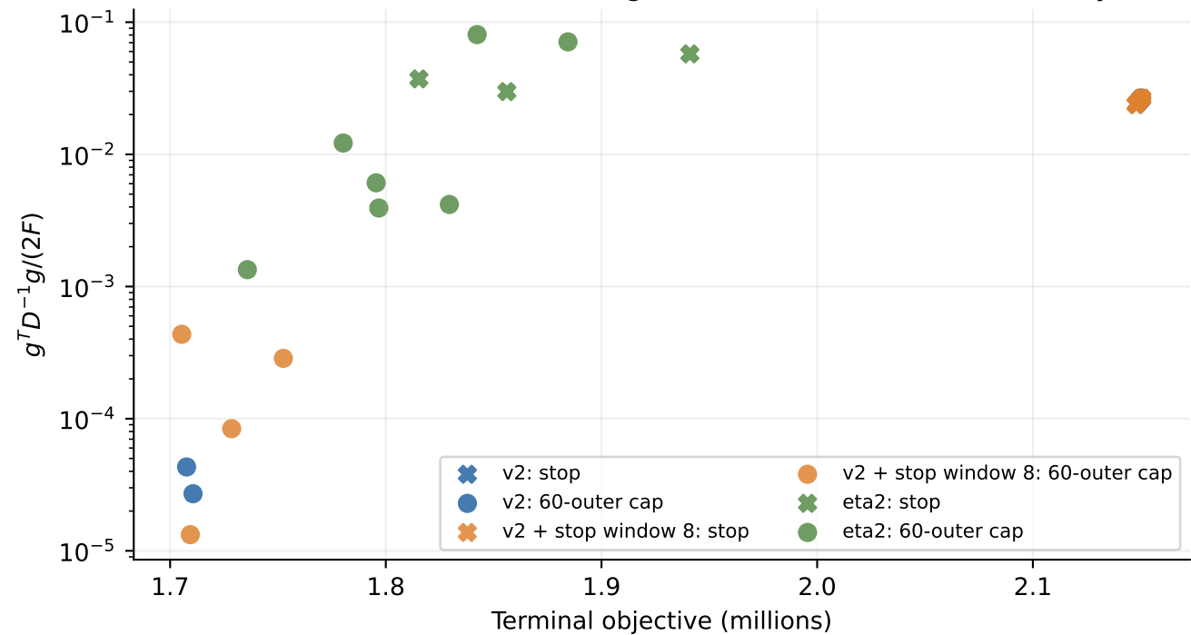
Final3068: a small cost change does not establish stationarity
