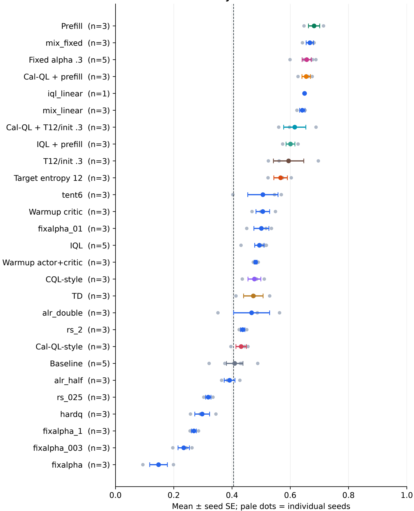
Early normalized AUC
