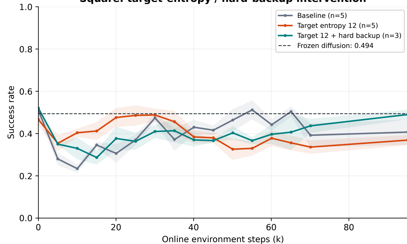
Square: target-entropy / hard-backup intervention
