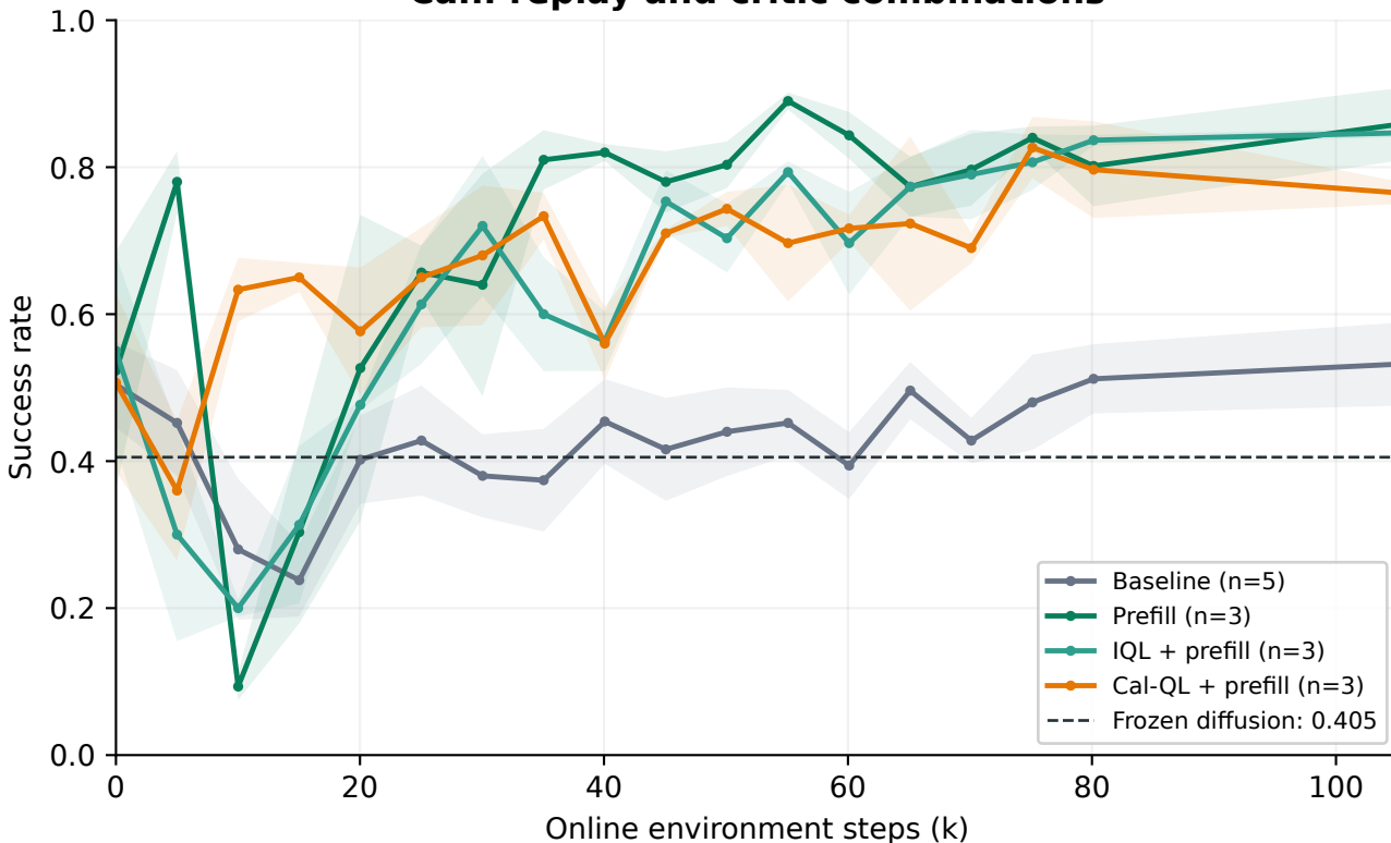
Square: late performance
