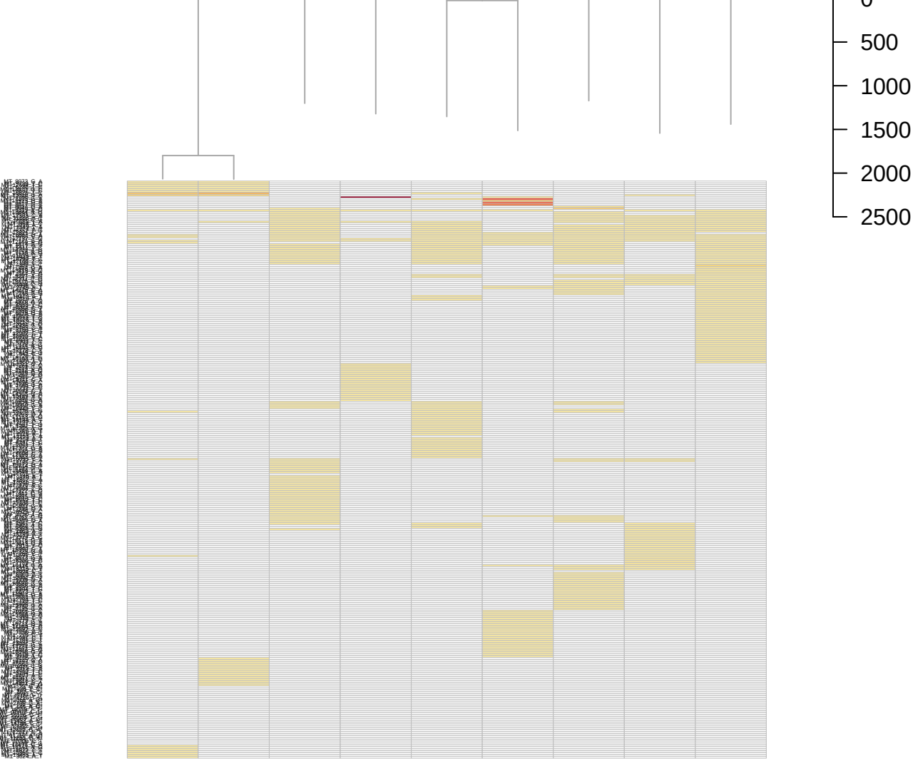
PD37595 (46 years old) : All mutations (VAF>0.1%)
