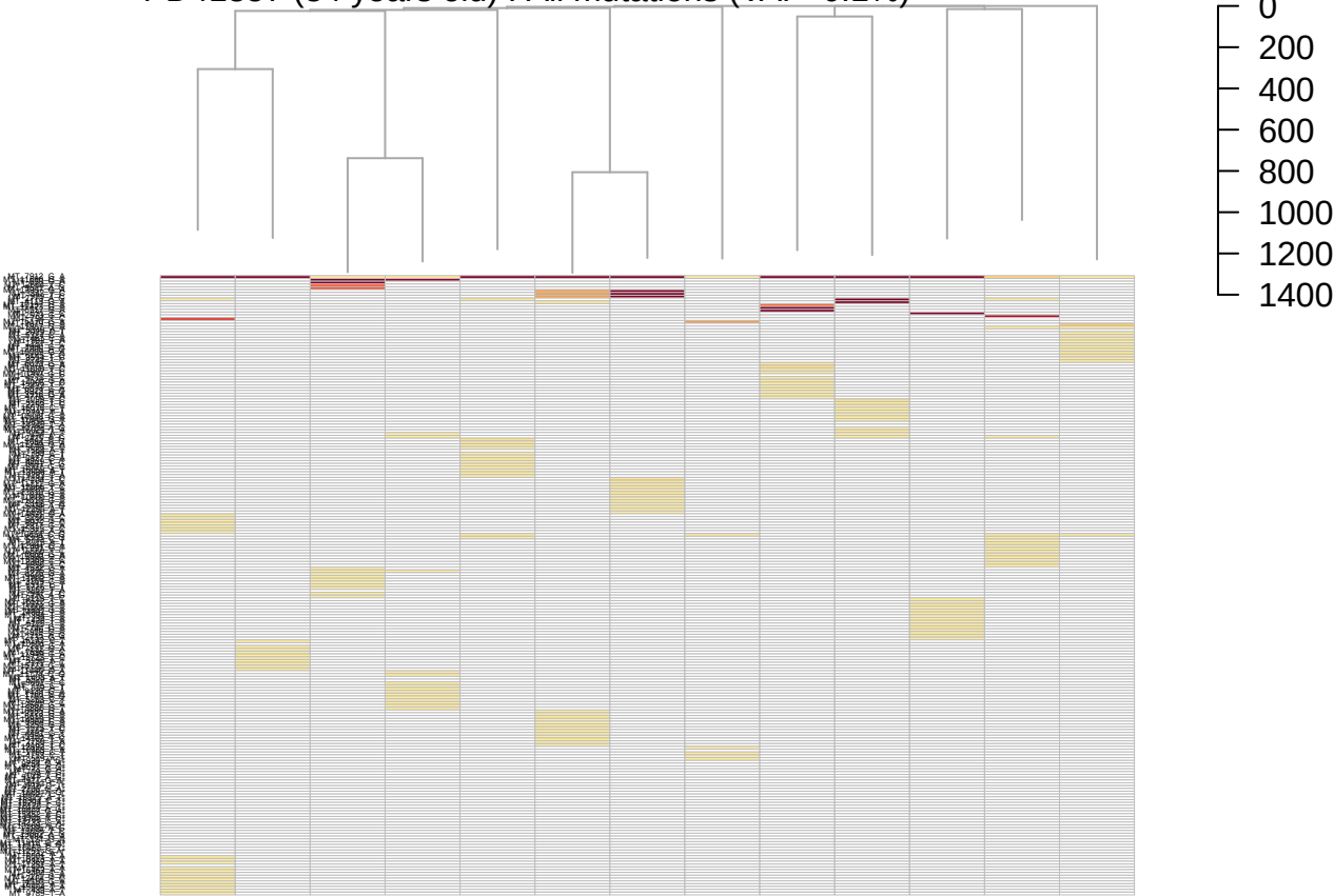
PD41857 (34 years old) : All mutations (VAF>0.1%)
