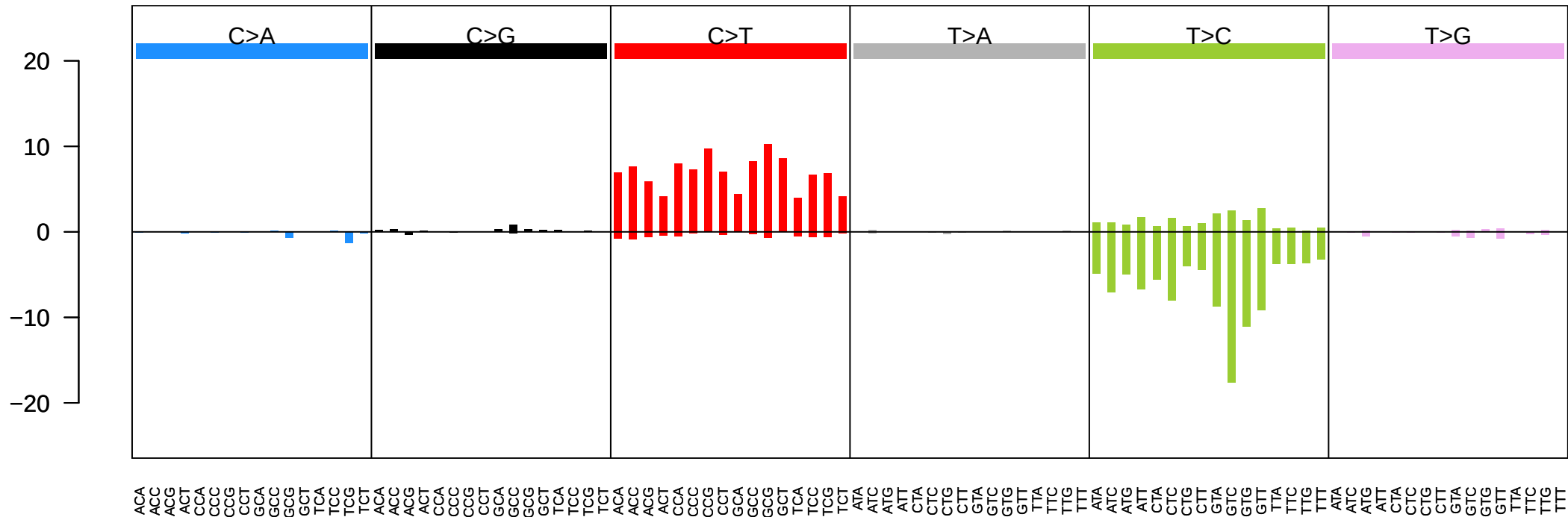
Mutation frequency (Obs/Exp)
