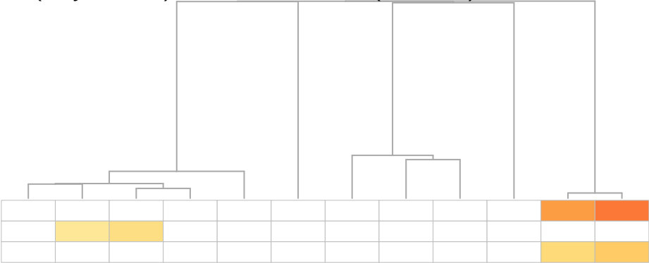
P29 (48 years old) : Shared mutations (VAF>3%)
