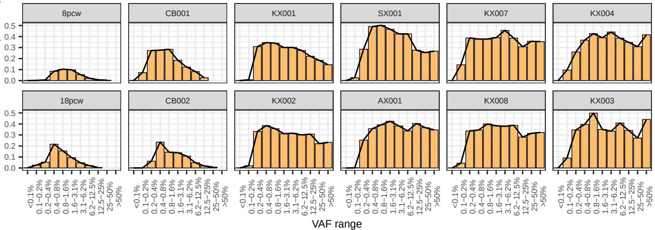
Number of N1 mutations detected per samp
