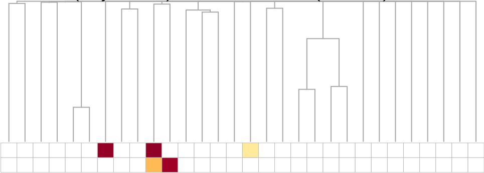
PD37449 (36 years old) : Shared mutations (VAF>3%)
