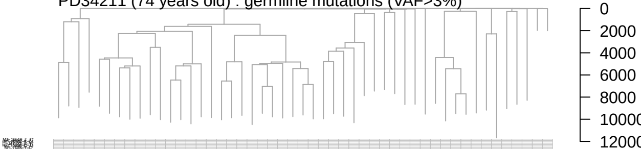
PD34211 (74 years old) : germline mutations (VAF>3%)
