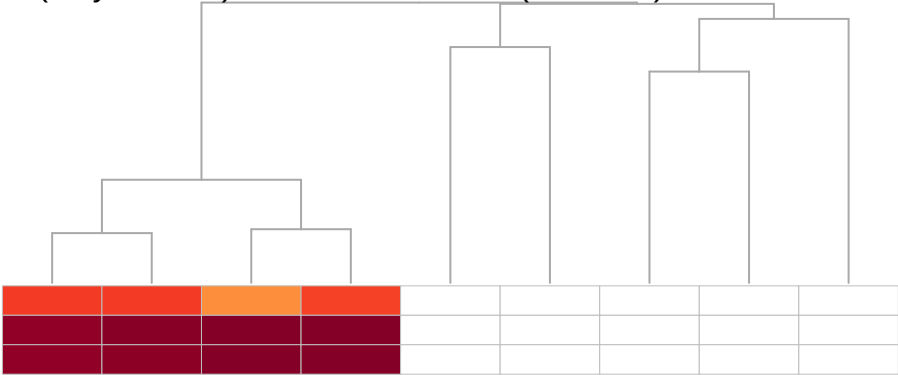
P41 (42 years old) : Shared mutations (VAF>3%)
