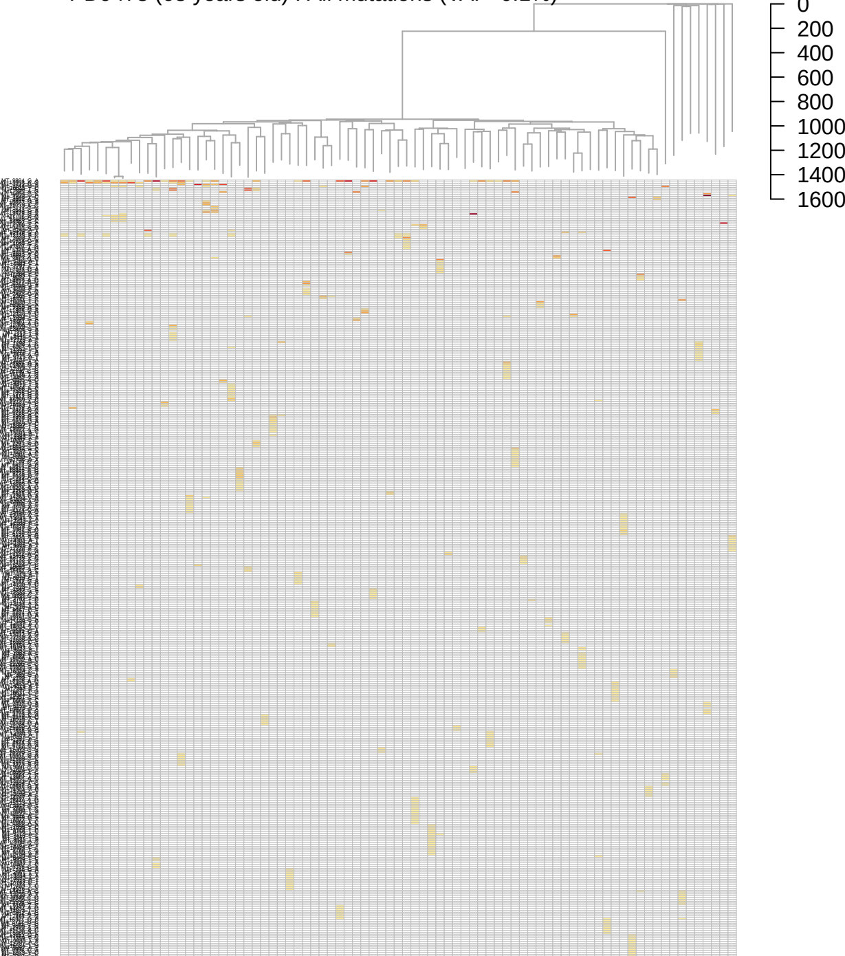
PD9478 (68 years old) : All mutations (VAF>0.1%)
