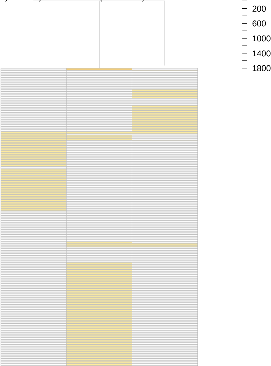
P19 (42 years old) : All mutations (VAF>0.1%)
