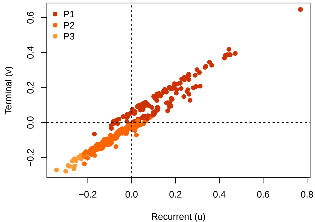
Frailty estimates by Ng and others
