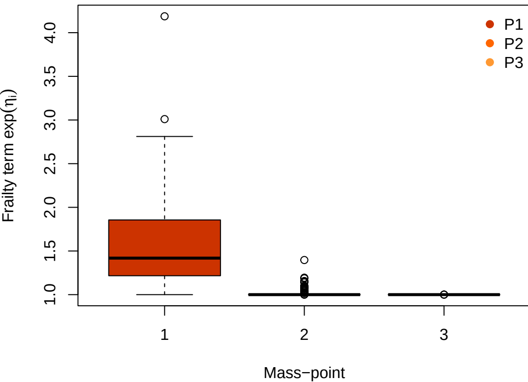
Frailty estimates by Rondeau and others
