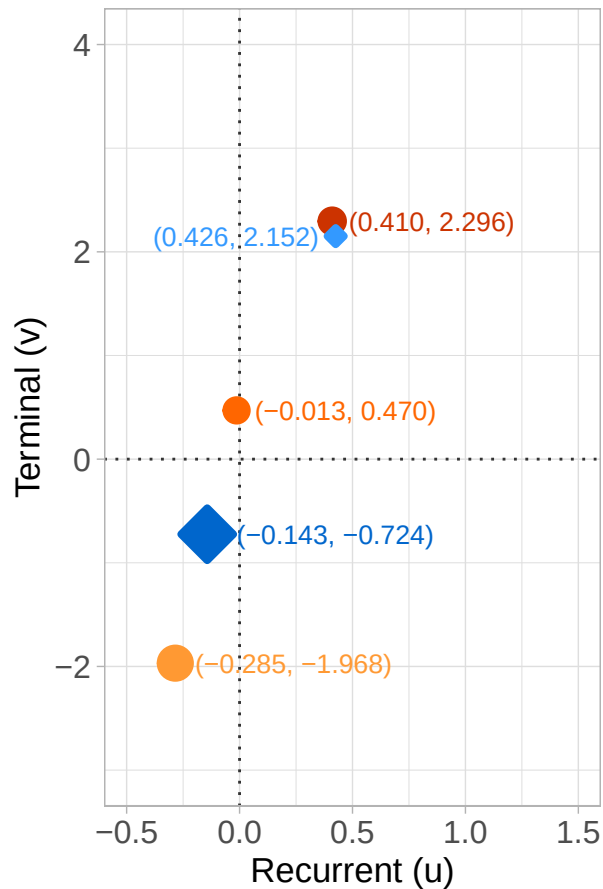
Mass distribution – Gaussian case
