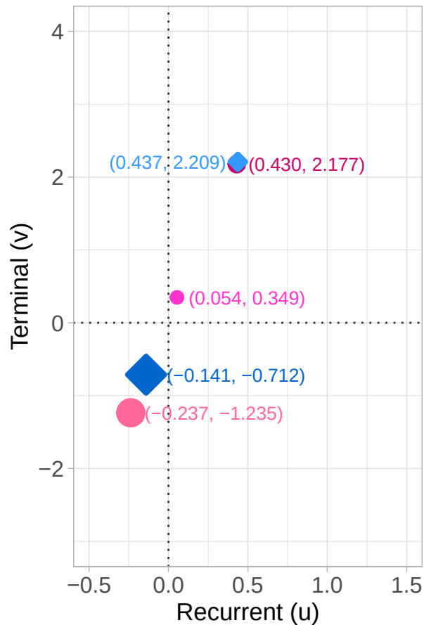
Mass distribution – Uniform case
