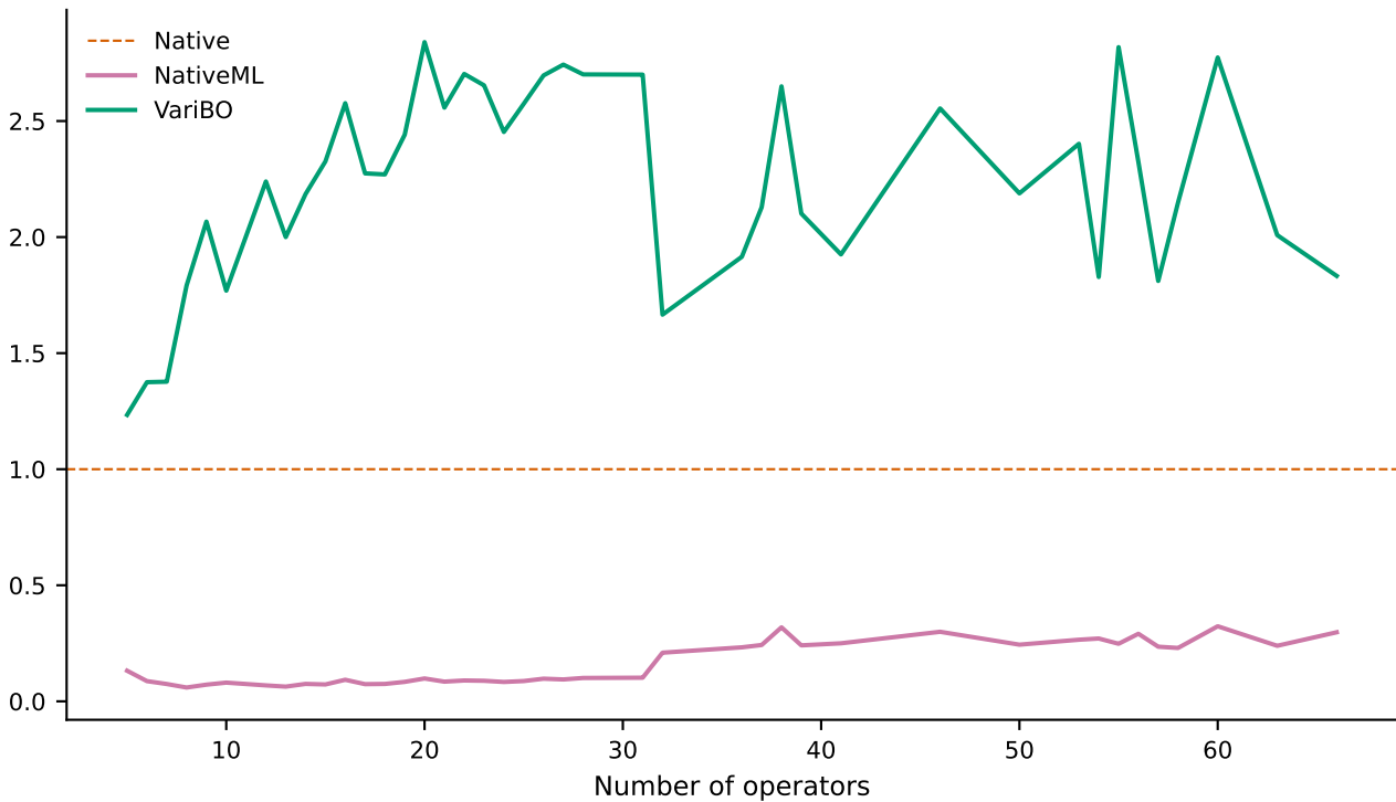
Speedup over Native
