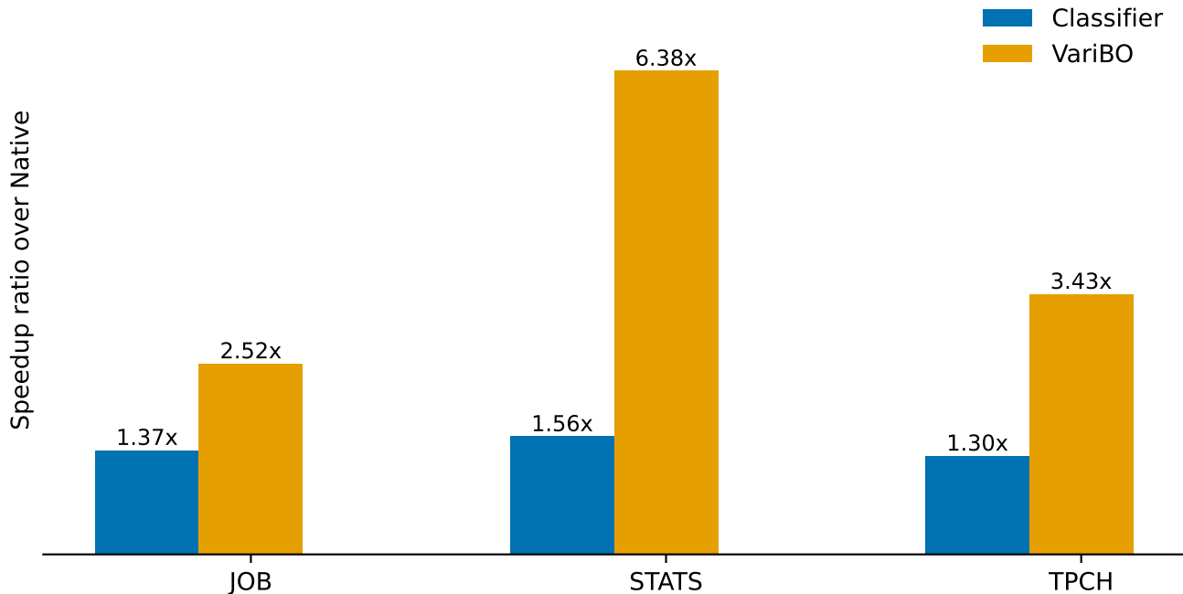
Speedup over Native in explored queries
