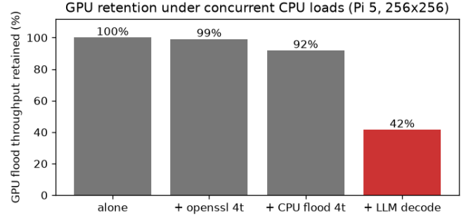
Fig. 2. GPU flood throughput retained beside three concurrent CPU loads, as a percentage of the same kernel running alone. Compute-bound and memory-bound CPU work barely disturb the GPU; language-model decode, which streams weights from DRAM every token, takes it to 42%. Raw logs in docs/paper/artifacts/ , genload2 and conc_steady .
