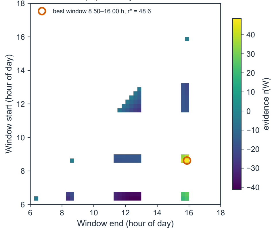
Evidence r(W) for every admissible window
