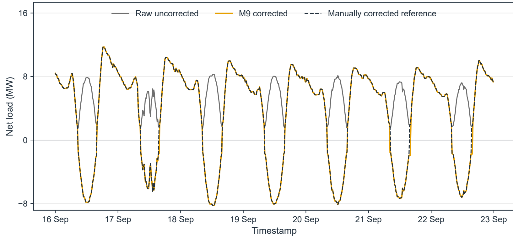
Highest-impact week of the test month (2024-09-16)
