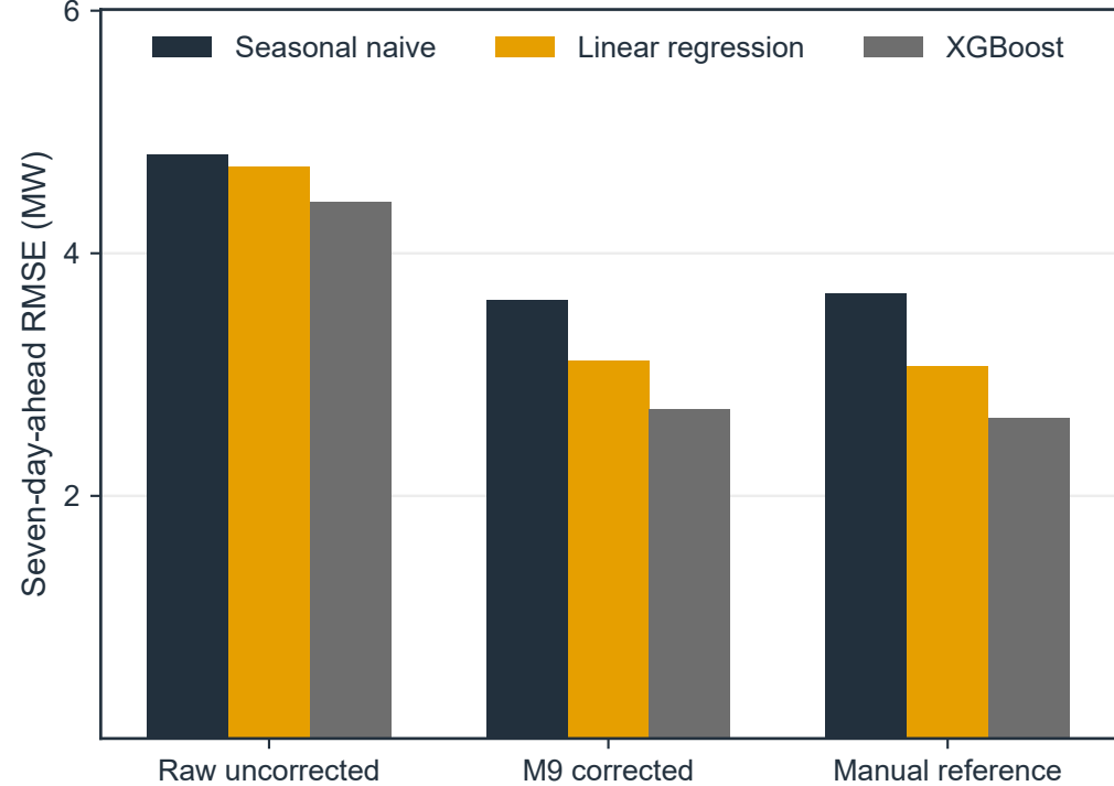
Direct point forecasts of the test month
