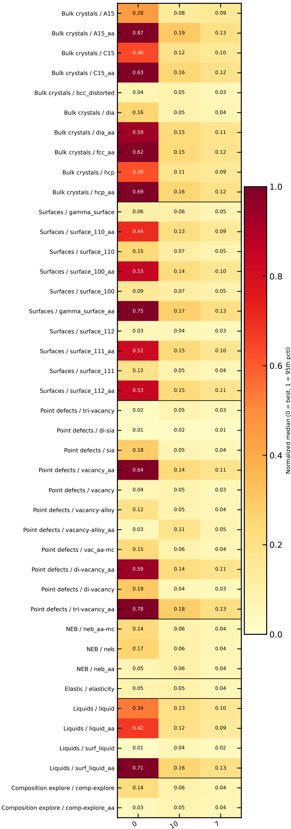
Force RMSE (eV/Å) — median across models
