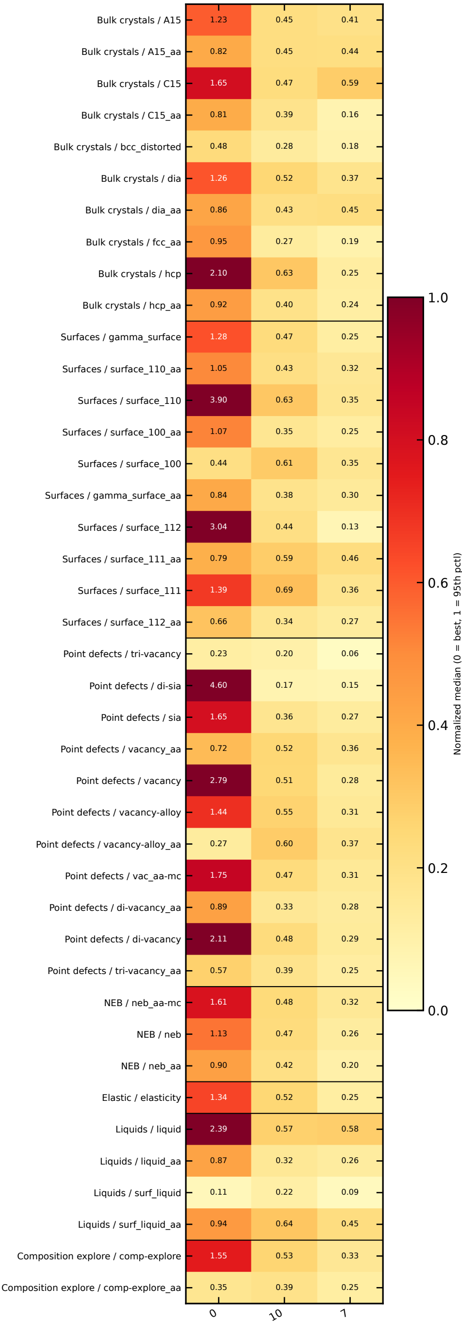
|\Delta P| (GPa) — median across models
