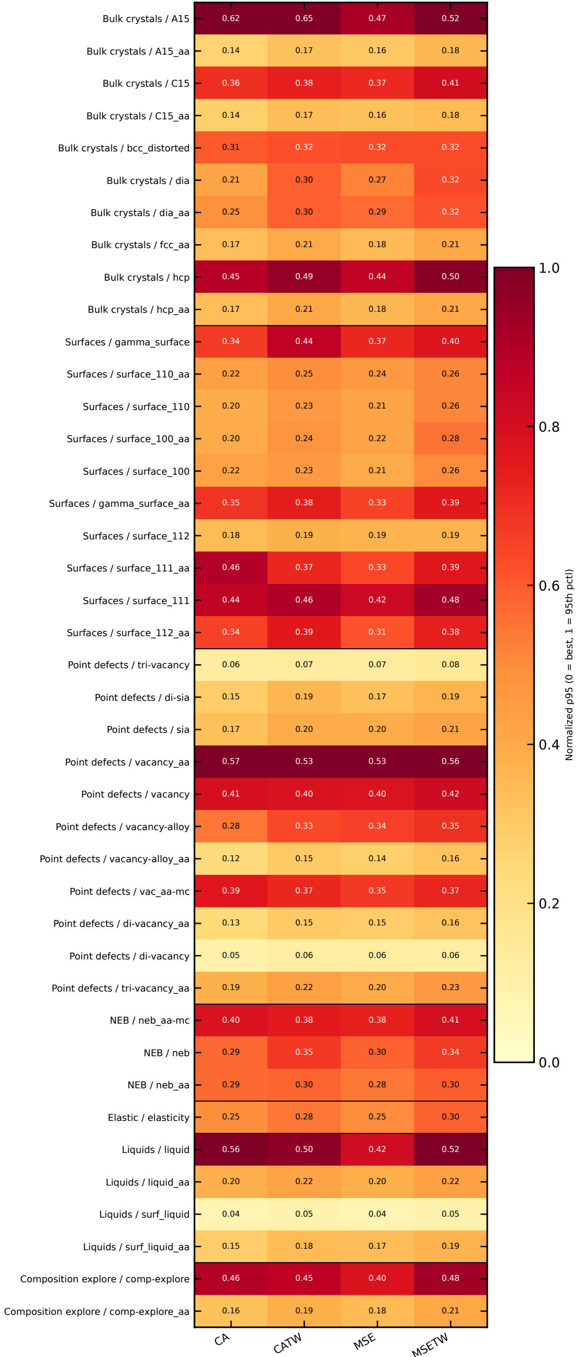
Force RMSE (eV/Å) — p95 across models
