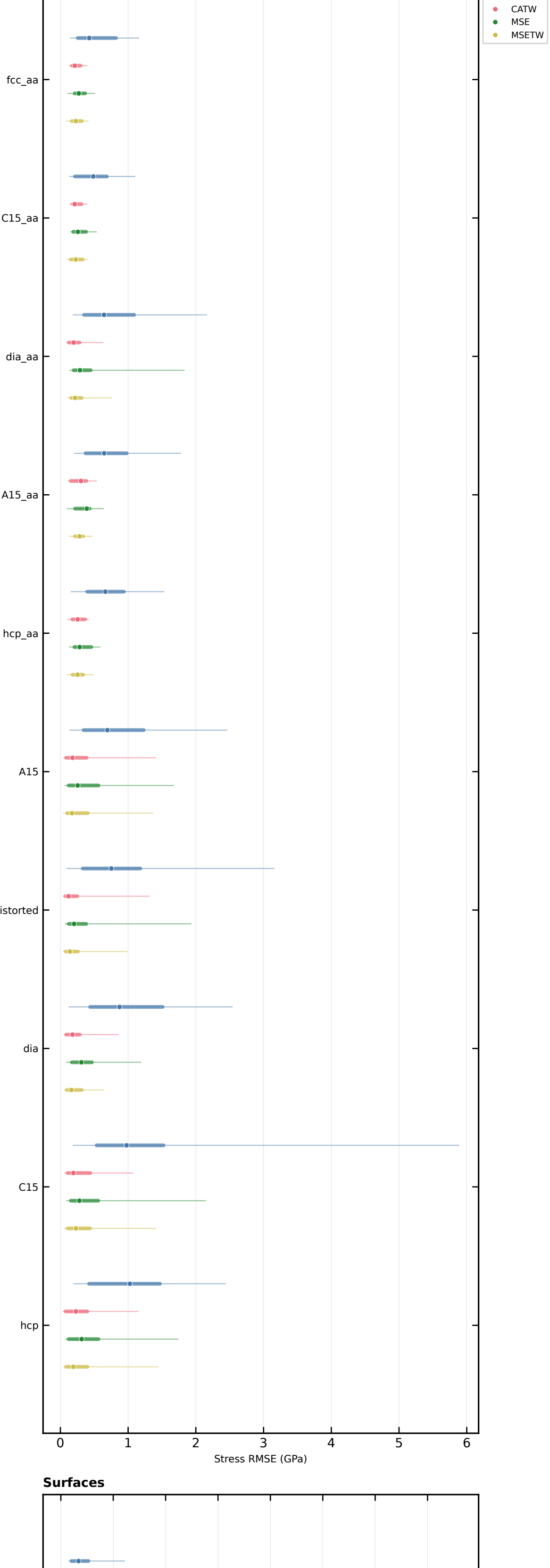
Stress RMSE (GPa) distribution by config_type (dot = median, thick = IQR, whisker = 5th-95th pct)
