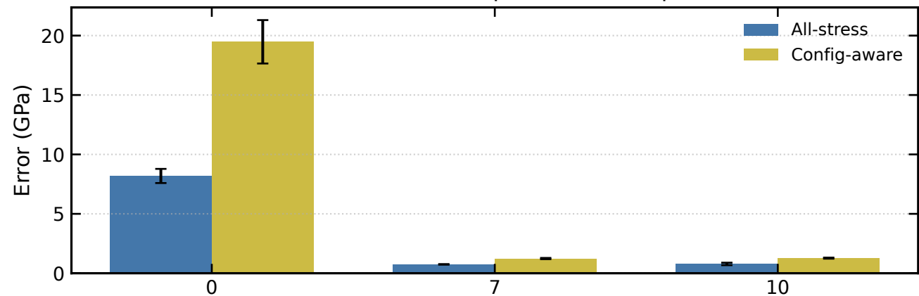
Generations — stress prediction comparison
