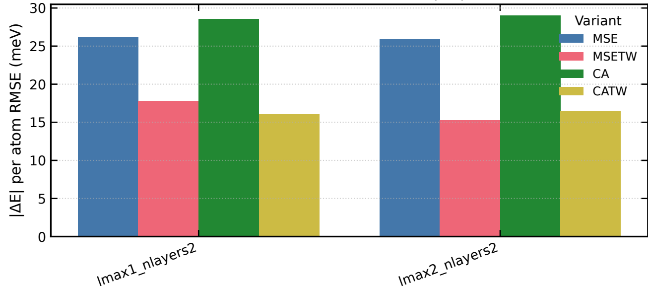
Loss variants across hyperparameter groups — |\Delta E| per atom RMSE (meV)
