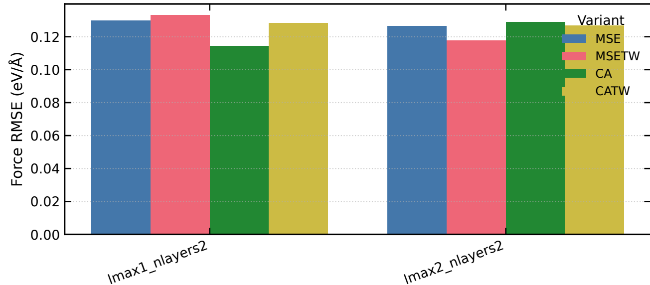
Loss variants across hyperparameter groups — Force RMSE (eV/Å)
