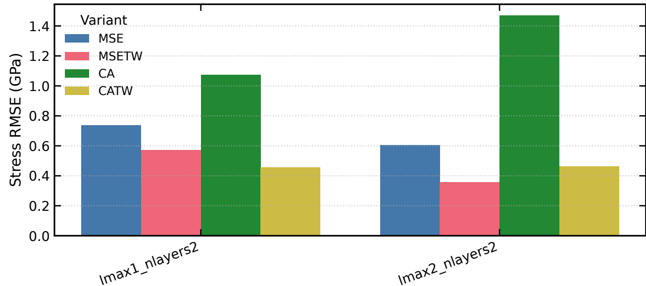
Loss variants across hyperparameter groups — Stress RMSE (GPa)
