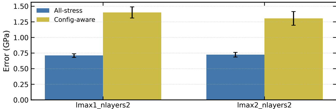
Loss groups — stress prediction comparison
