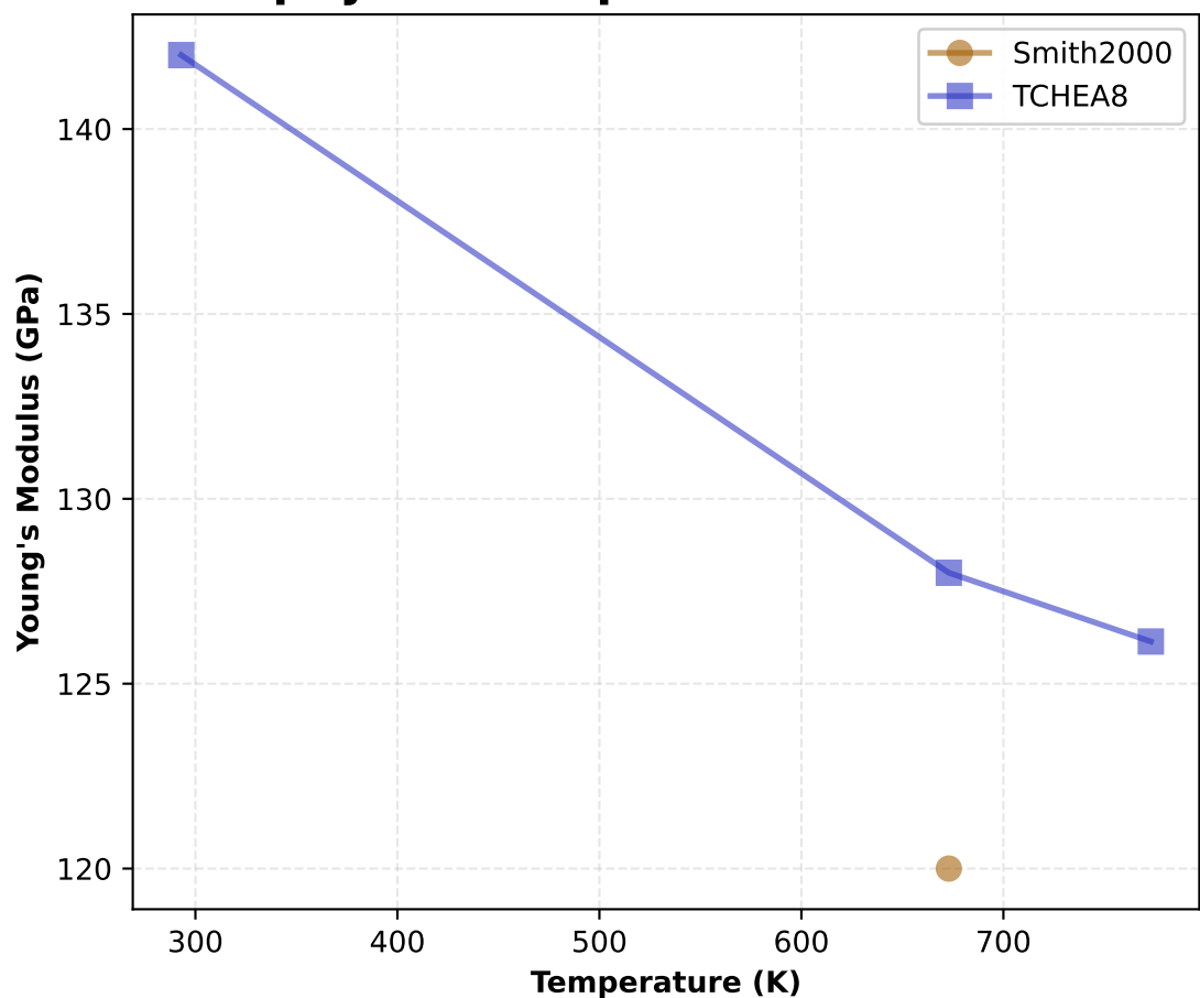
TCHEA8 vs Smith2000: V-4Cr-4Ti Thermophysical Properties
