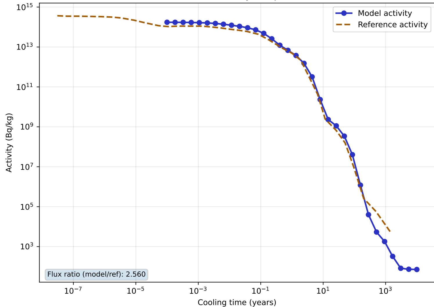
V-15Cr-5Ti activity comparison
