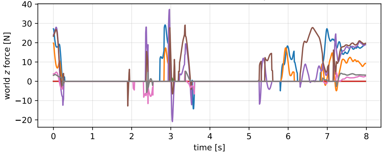
World-frame vertical force component f_z
