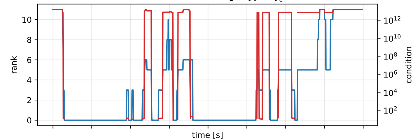
Rank and conditioning of J_c M^{-1} J_c^T
