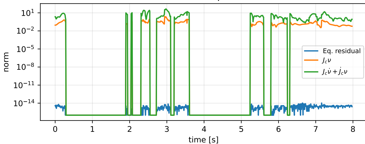
Fixed-contact assumption residuals
