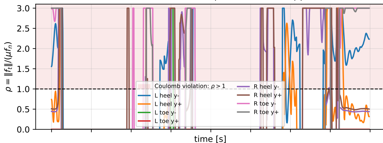
Friction ratio; shaded when \rho > 1 (values clipped at 3)
