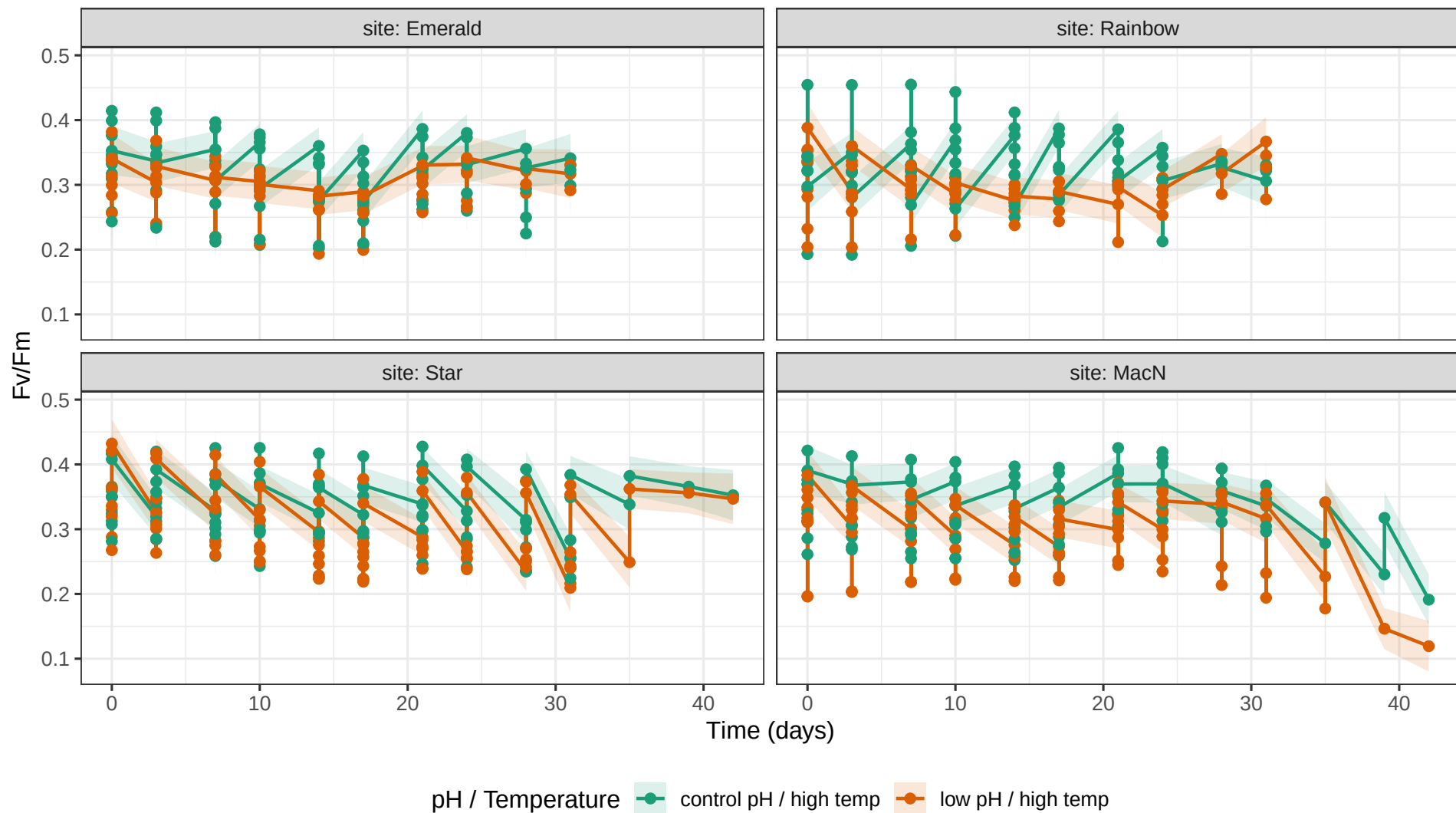
Fitted Fv/Fm trajectories – ssid_heat
