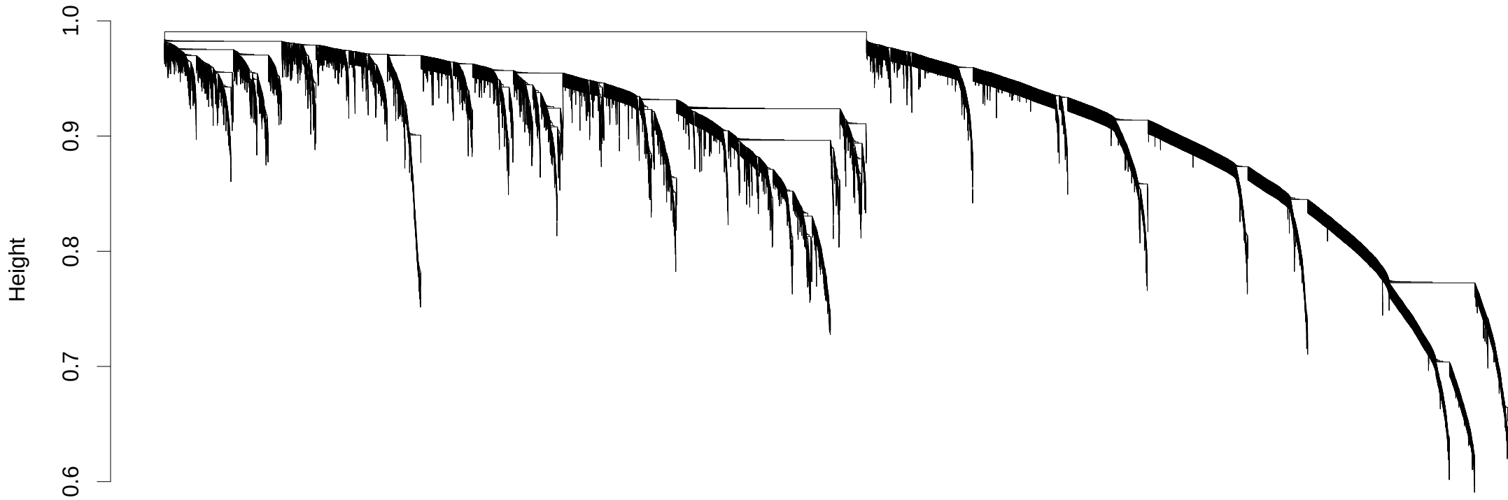
Cluster Dendrogram
