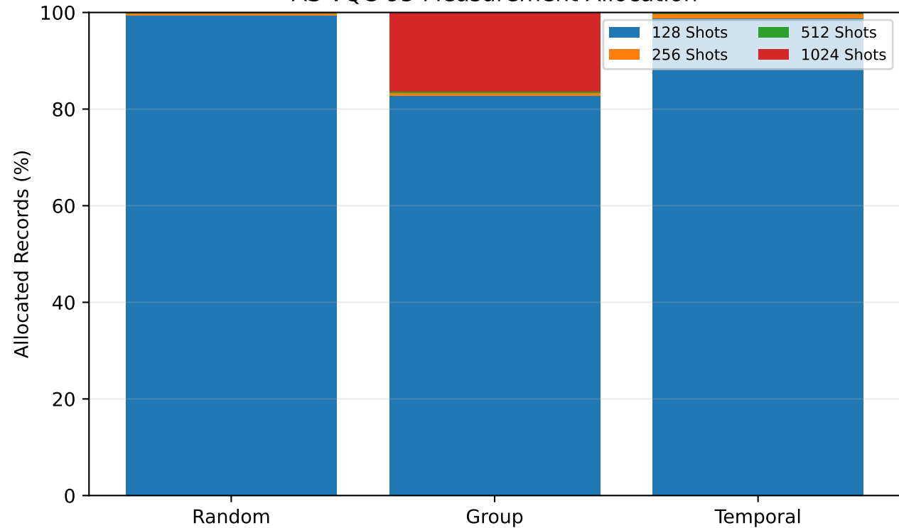
AS-VQC-95 Measurement Allocation
