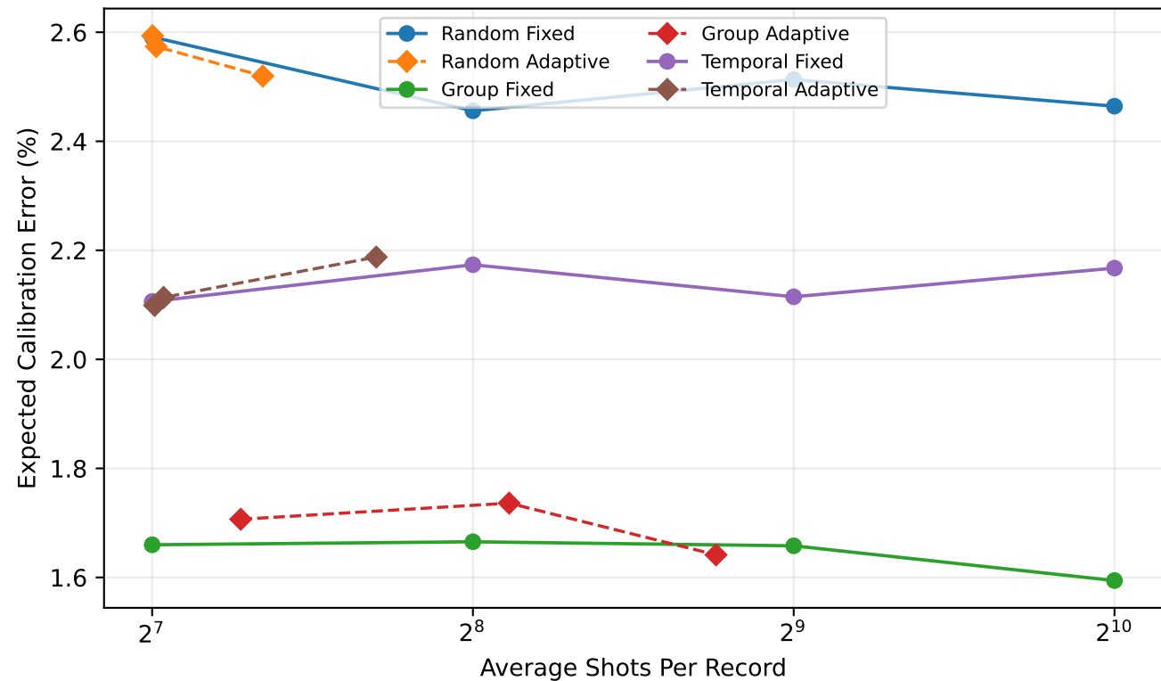
Calibration-Measurement Trade-Off
