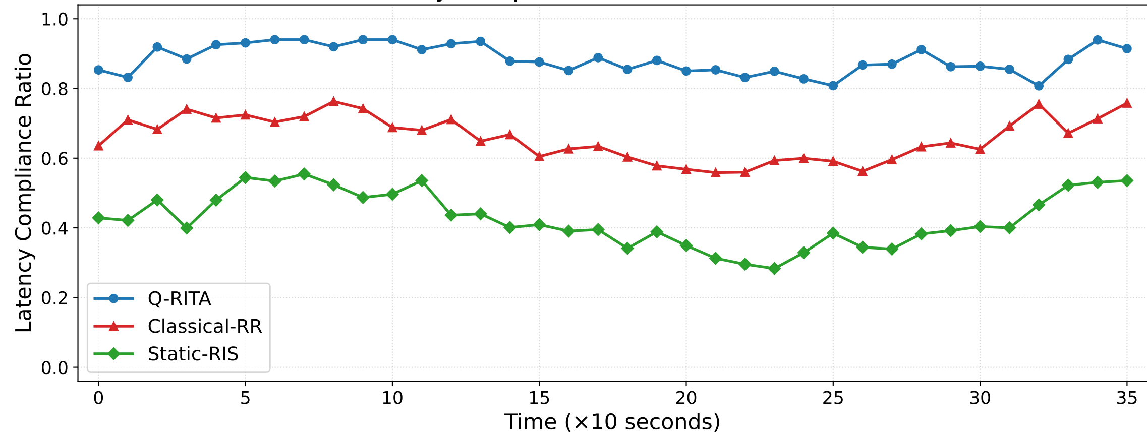
Latency Compliance Ratio (LCR) over Time
