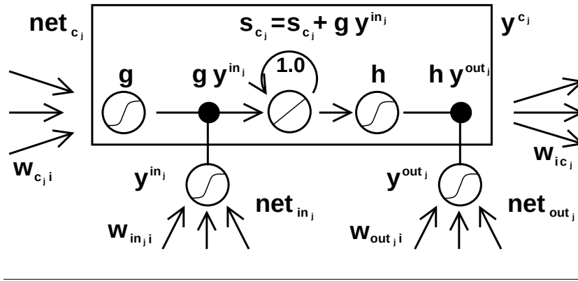
Figure 1: Architecture of memory cell c_j (the box) and its gate units in_j, out_j . The self-recurrent connection (with weight 1.0) indicates feedback with a delay of one time step. It builds the basis of the CEC. The gate units open and close access to CEC. See text and appendix A.1 for details.
