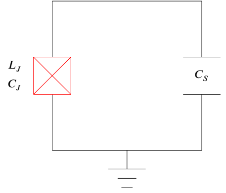
Figure 1: Illustration of Josephson qubit circuit[79]. L_J is the “nonlinear inductance” and is “shunted” by a capacitance, C_S . L_J , C_J , and the red hatched box is a substitute for a single inductor L in order that the separation between the ground state |0\rangle , first excited state, |1\rangle , second excited state, |2\rangle , etc. are not evenly spaced.
