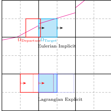
Figure 1: Illustration of the Eulerian Implicit, Lagrangian Explicit cell integrated semi-Lagrangian (CISL) method[21, 38]. Rather than have separate traversals through the grid for the cell-centered, face centered, and edge centered variables, we instead interpolate all variables to a refined grid, followed by one traversal through the refined grid, and then conservatively average the respective results back to their defined control volumes.
