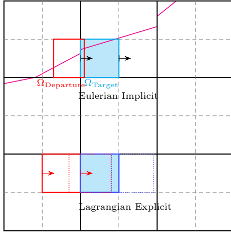
Figure 1: Illustration of the Eulerian Implicit, Lagrangian Explicit cell integrated semi-Lagrangian (CISL) method[21, 39]. Rather than have separate traversals through the grid for the cell-centered, face centered, and edge centered variables, we instead interpolate all variables to a refined grid, followed by one traversal through the refined grid, and then conservatively average the respective results back to their defined control volumes.
