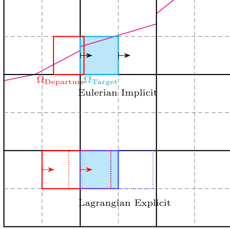
Figure 1: Illustration of the Eulerian Implicit, Lagrangian Explicit cell integrated semi-Lagrangian (CISL) method[26, 46]. Rather than have separate traversals through the grid for the cell-centered, face centered, and edge centered variables, we instead interpolate all variables to a refined grid, followed by one traversal through the refined grid, and then conservatively average the respective results back to their defined control volumes.
