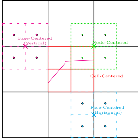
Figure 3: After Cell Integrated Semi-Lagrangian advection[26, 47] on the refined grid, the cell centered variables, F_m , \phi_m , and E_m , and the face centered variables, (u, v) , are conservatively “recombined” back to their respective control volume locations. The deviatoric stress tensor components, s_m^{xx,yy,\Theta\Theta} (RZ), are conservatively recombined to the cell centered control volumes, and then piecewise constant prolonged back to the refined grid. The off-diagonal deviatoric stress tensor component, s_{xy} , is conservatively recombined to the node control volume (RZ) (edge centers in 3D), and then piecewise constant prolonged back to the refined grid. The material density, \rho_m , do not need to be recombined.
