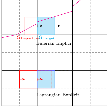
Figure 1: Illustration of the Eulerian Implicit, Lagrangian Explicit cell integrated semi-Lagrangian (CISL) method[26, 47]. Rather than have separate traversals through the grid for the cell-centered, face centered, and edge centered variables, we instead interpolate all variables to a refined grid, followed by one traversal through the refined grid, and then conservatively average the respective results back to their defined control volumes.
