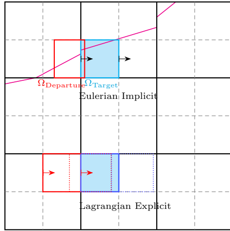
Figure 1: Illustration of the Eulerian Implicit, Lagrangian Explicit cell integrated semi-Lagrangian (CISL) method[?, ?]. Rather than have separate traversals through the grid for the cell-centered, face centered, and edge centered variables, we instead interpolate all variables to a refined grid, followed by one traversal through the refined grid, and then conservatively average the respective results back to their defined control volumes.
