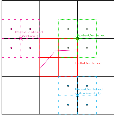
Figure 3: After Cell Integrated Semi-Lagrangian advection[?, ?] on the refined grid, the cell centered variables, F_m , \phi_m , and E_m , and the face centered variables, (u, v) , are conservatively “recombined” back to their respective control volume locations. The deviatoric stress tensor components, s_m^{xx,yy,\Theta\Theta} (RZ), are conservatively recombined to the cell centered control volumes, and then piecewise constant prolonged back to the refined grid. The off-diagonal deviatoric stress tensor component, s_{xy} , is conservatively recombined to the node control volume (RZ) (edge centers in 3D), and then piecewise constant prolonged back to the refined grid. The material density, \rho_m , do not need to be recombined.
