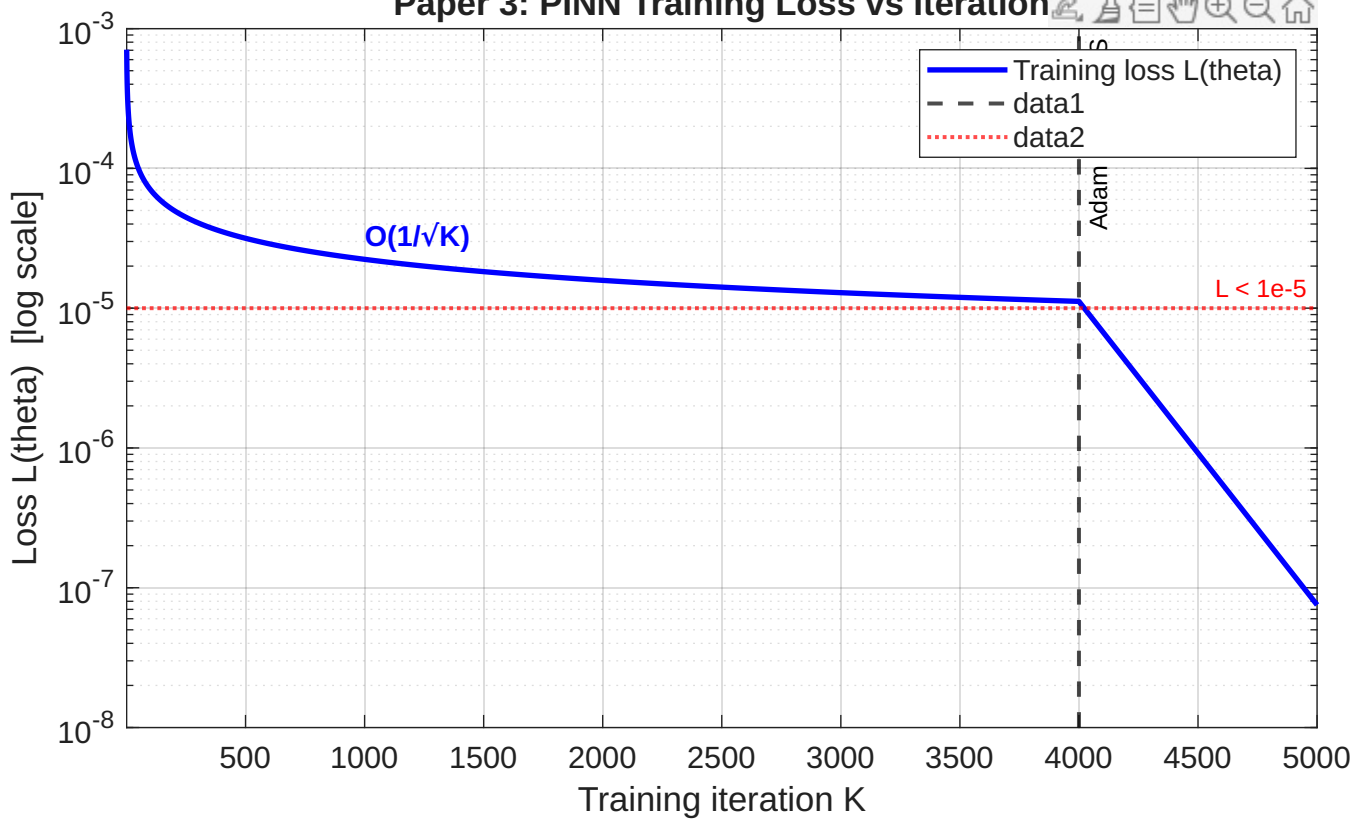
Paper 3: PINN Training Loss vs Iteration
